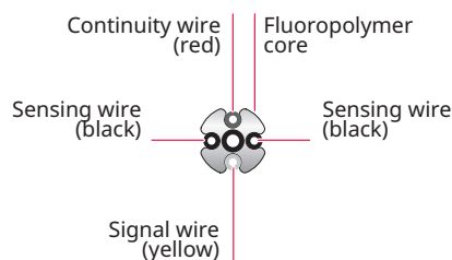
Cable construction
